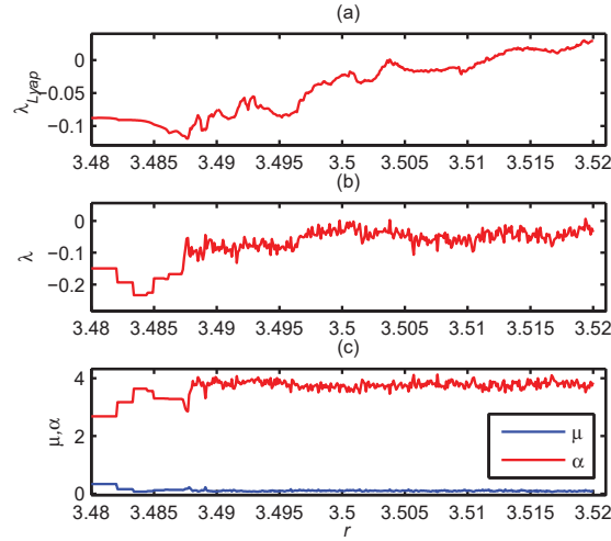
Figure 4.19: Detection of the transition from torus to SNA by the H-H route in the forced logistic map, \epsilon = 0.3 , n = 3 , 4 \leq \phi \leq 13 , T = 10^6 . From top to bottom the Lyapunov exponent, the non-regularity index \lambda and the regularity indices \mu and \alpha .
