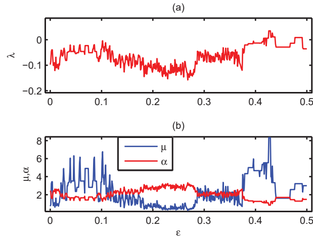
Figure 4.14: OA growth indices spectra for SNA detection in the GOPY with r = 1.5 and 0 \leq \epsilon \leq 0.5 . We set T = 2 \times 10^4 , n = 2 and 9 \leq \phi \leq 18 ( 11 \leq \rho \leq 20 ).
