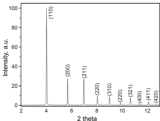
Figure 7. Diffraction pattern of an EBM-processed cp-Fe obtained by HE-XRD at the PETRA III synchrotron source.
