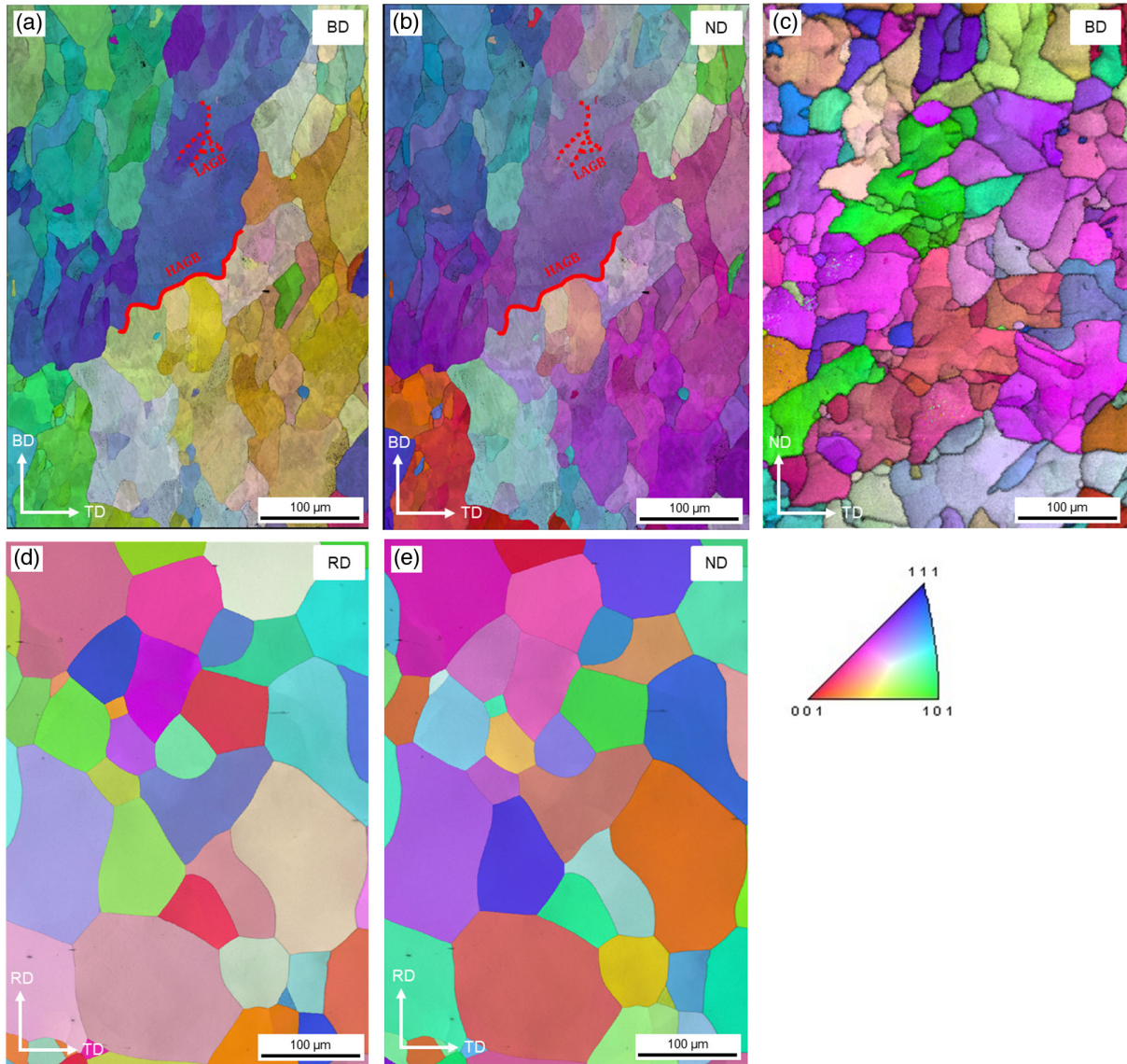
Figure 4. EBSD analysis (inverse pole figure maps): a) EBM-processed cp-Fe in side view plotted with respect to BD and b) normal direction; c) top view indexed with respect to BD. d,e) HR Fe plotted with respect to (d) rolling direction and (e) normal direction.
