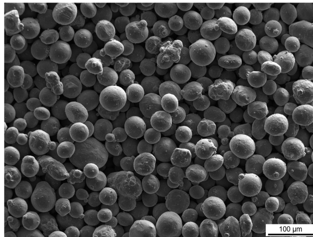
Figure 1. SEM micrograph of the cp-Fe powder.
