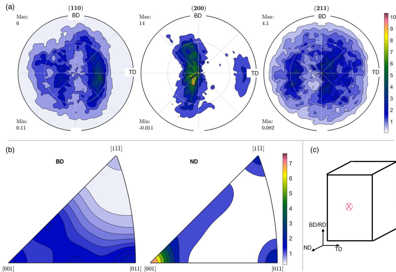
Figure 6. a) Pole figures for EBM-processed cp-Fe; b) inverse pole figures calculated for the same surface; c) schematic indicating the probed spot by the red "X."
